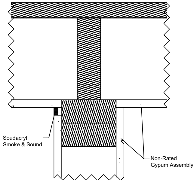
1" (6.35mm) Thickness Both Sides of Wall
